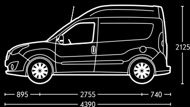
Combo Cargo L1H2.
